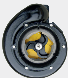
Shearing impeller
